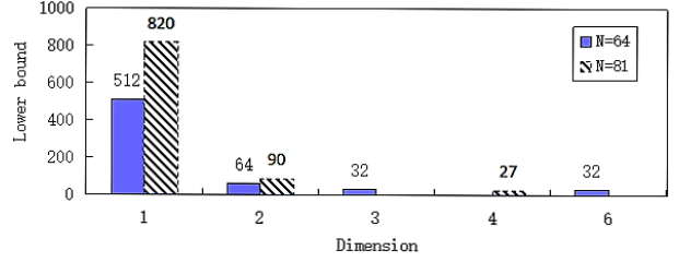
Figure 3: Lower bound of wavelengths when N is fixed
